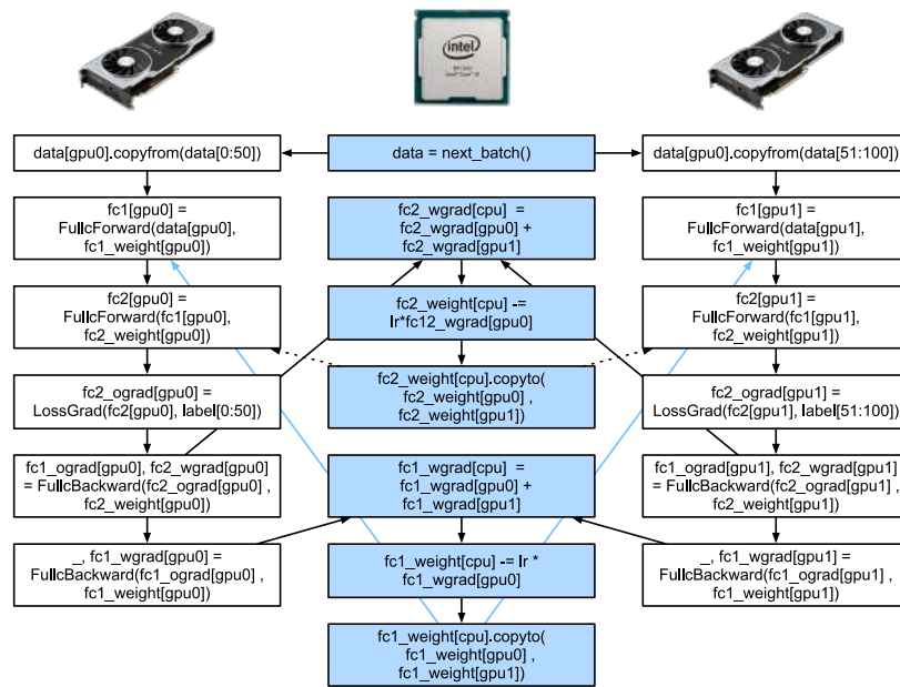
Fig. 13.3.1 The computational graph and its dependencies of a two-layer MLP on a CPU and two GPUs.
